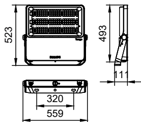
BVP433 LED522/CW 220~240V 380W S6 GM
